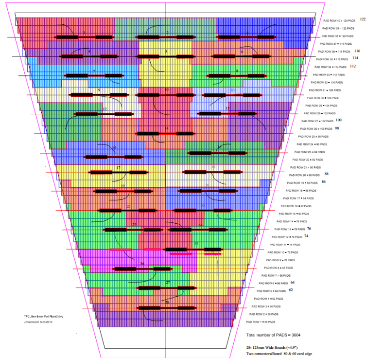
Figure 74: The new padplane design
