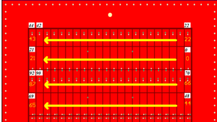
Figure 45: Pad numbering scheme for the small MWPC prototype.
