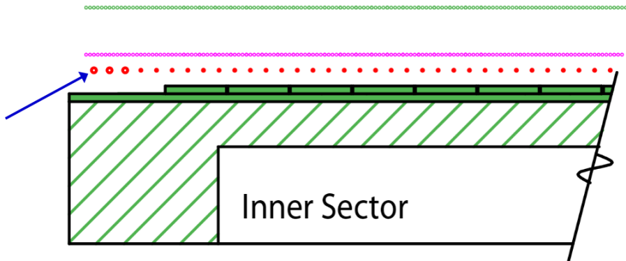
Figure 38: Three low gain wires (125 \mu\text{m} diameter) will be placed on both ends of the anode wire grid. The low gain wires will reduce the production of ions in the region where they can leak into the drift-volume of the TPC. Another option is to ground the last wire so that the gain is zero on that wire.
