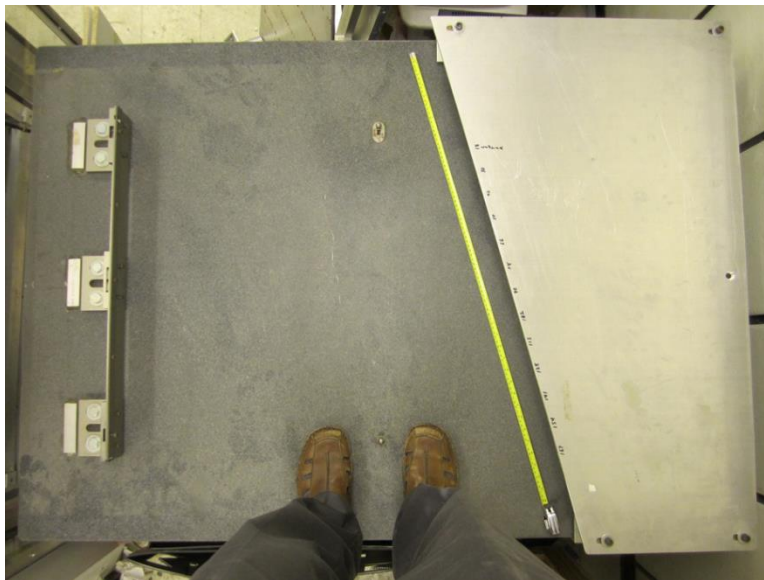
Figure 63: Top view of a granite table with one of the wire alignment combs exposed. The second comb lies under the aluminum shield on the right. Scale: the yellow portion of the tape is 1 meter long.
