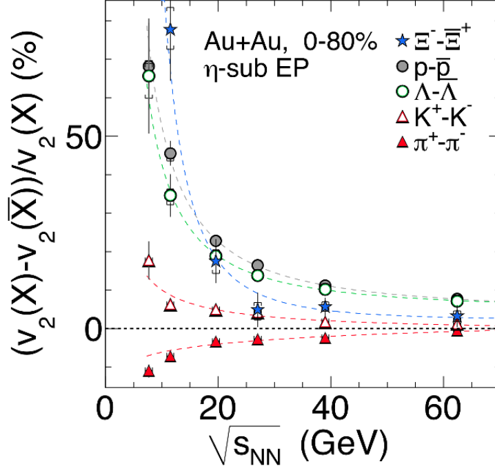
Figure 9: The difference in v_2 between particles and their antiparticles (see legend) as a function of \sqrt{s_{\text{NN}}} for 0-80% central Au+Au collisions. The dashed lines are fits with a power-law function. The error bars depict the combined statistical and systematic errors.
