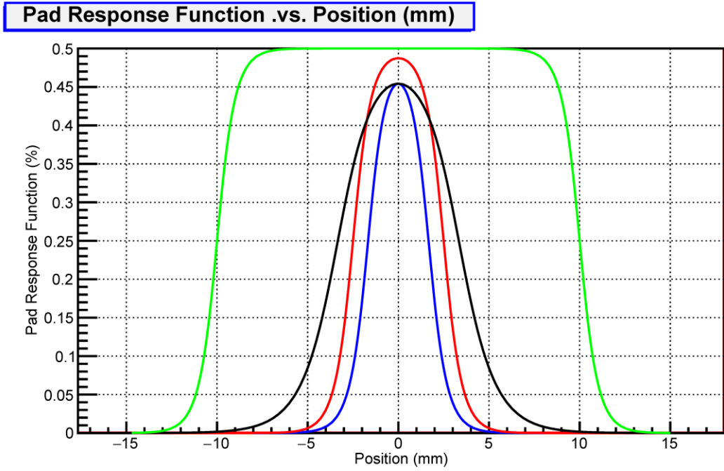
Figure 33: The pad response function for the outer sector is shown by the black line, the existing inner sector by the blue line, and the proposed inner sector by the red line. The pad spacing is 6.7 mm, 3.35 mm, and 5 mm respectively. The padplane to anode wire plane distance is 4 mm in the outer sector and 2 mm in the inner sector. The green line shows the PRF for a very wide pad, 20 mm, and it suggests that 50% of the signal goes to the padplane in the asymptotic limit. The diffusion width for an electron that drifts the full length of the TPC would be a curve that lies very close to the black line.
