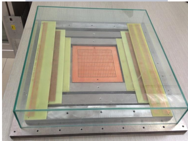
Figure 43: Exploded view and setup for the small scale MWPC prototype.
