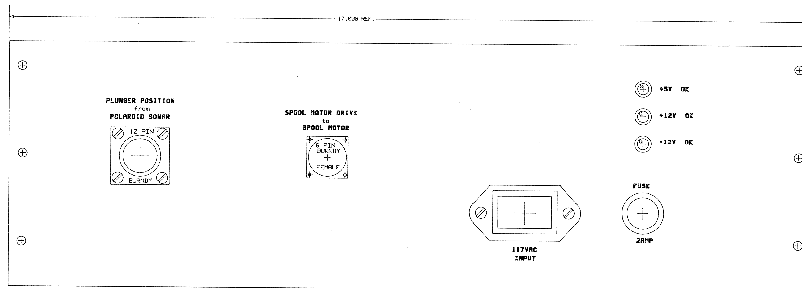
REAR PANEL
