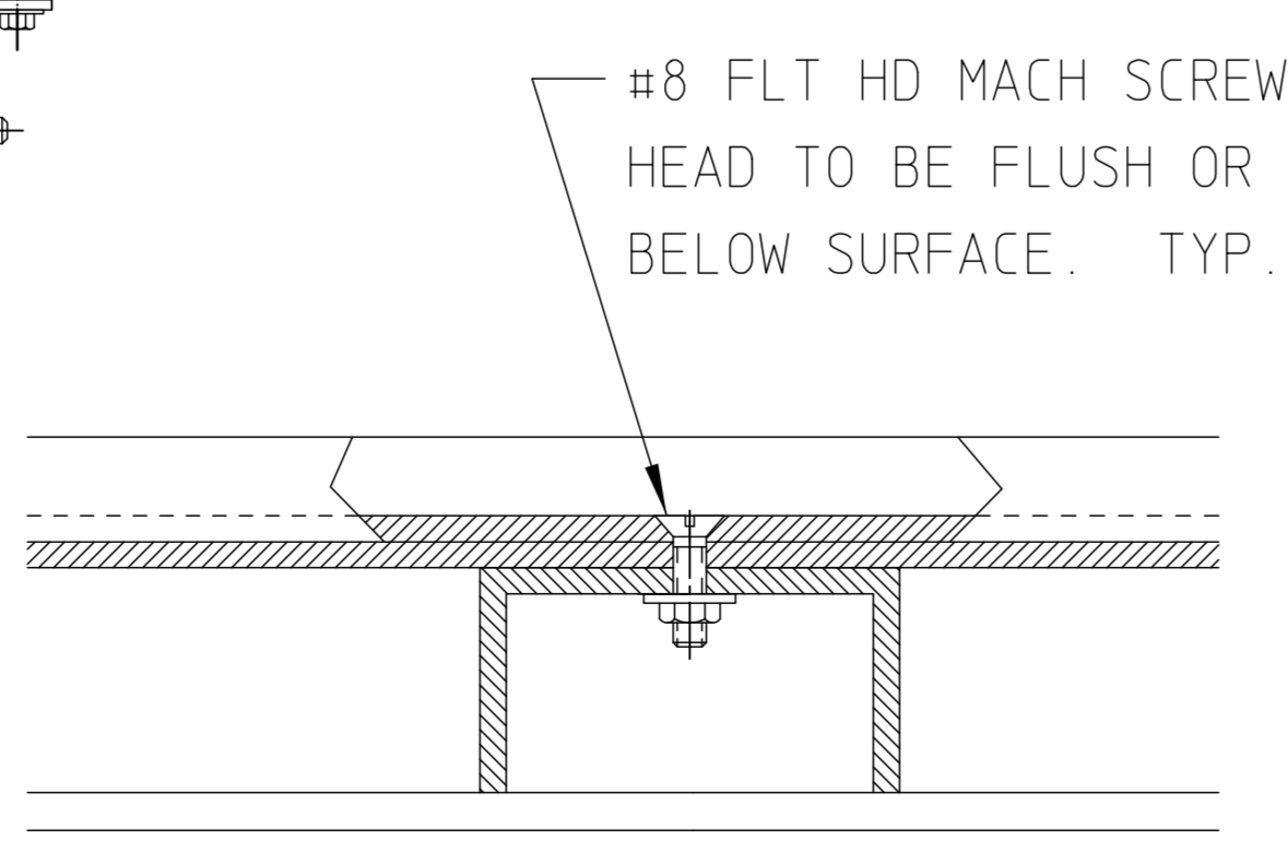
DETAIL "B" TRACK HOLD-DOWN SCALE: FULL SIZE
