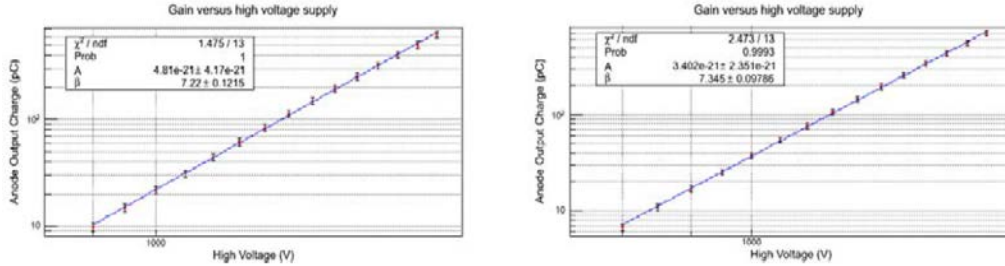
Figure 68: the anode output charge versus high voltage supply of Hamamatsu R11102-A52468 (left) and R11102-A52723 (right).
