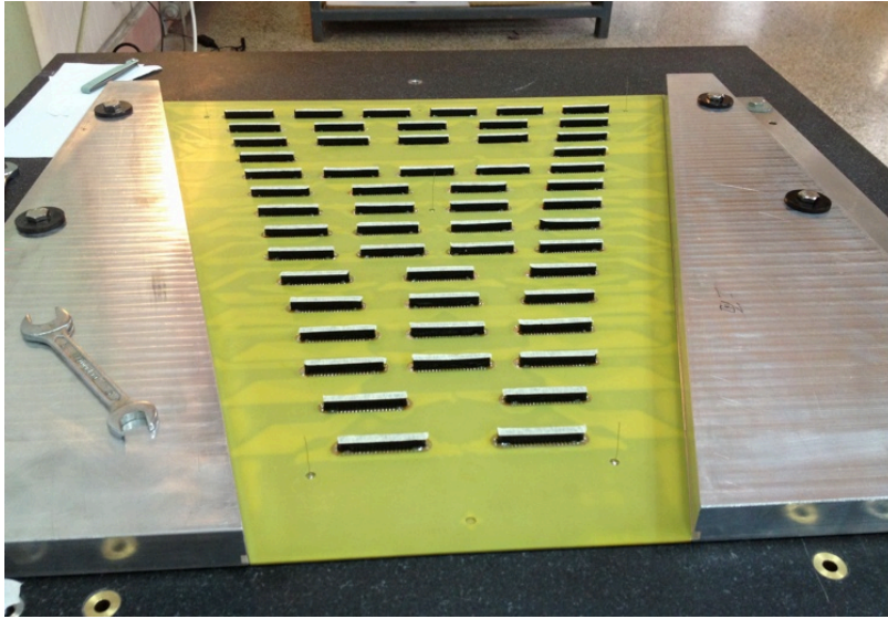
Figure 73: Padplane on granite table held flat by the suction of a vacuum system.
