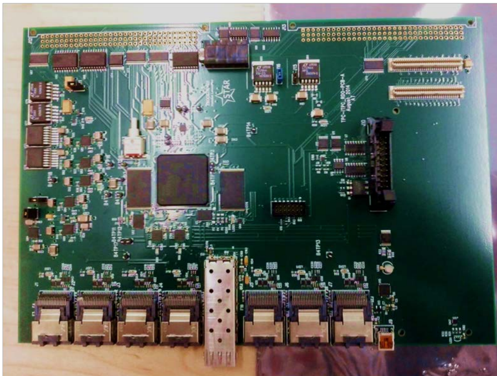
Figure 90: iRDO prototype.
