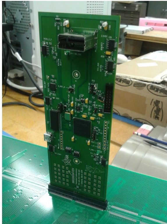
Figure 89: Pre-prototye iFEE (ppFEE) electronic card shown plugged into the padplane
