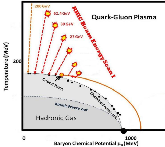
Figure 15: A schematic version of the QCD phase diagram. Overlaid are conceptual illustrations of reaction trajectories for central collisions.
