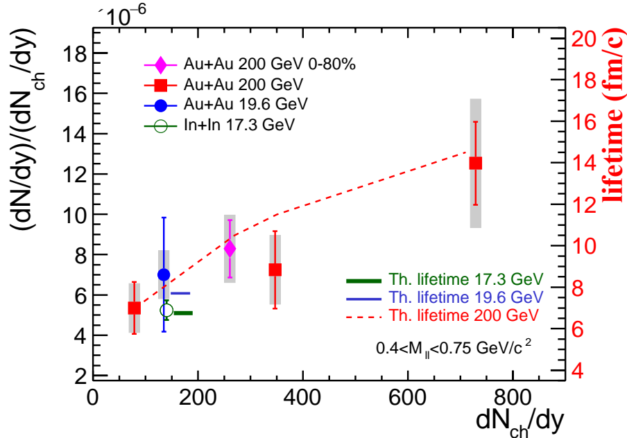
Figure 9: Integrated yields of the normalized dilepton excesses for 0.4 < M_{II} < 0.75 \text{ GeV}/c^2 as a function of dN_{ch}/dy . The solid circle and diamond represent the results in 0-80% Au+Au collisions at \sqrt{s_{NN}} = 19.6 and 200 GeV, respectively. The squares are the results for 40-80%, 10-40%, and 0-10% Au+Au at \sqrt{s_{NN}} = 200 GeV. The open circle represents the dimuon result from the NA60 measurement with dN_{ch}/dy > 30 . Bars are statistical uncertainties, and systematic uncertainties are shown as grey boxes. The theoretical lifetimes for \sqrt{s_{NN}} = 200 GeV Au+Au as a function of dN_{ch}/dy in the model calculations [37] are shown as a dashed curve. The lifetimes for \sqrt{s_{NN}} = 17.3 GeV In+In and \sqrt{s_{NN}} = 19.6 GeV Au+Au in the same model calculations [37] are shown as the two horizontal bars. The dN_{ch}/dy values for the horizontal bars are shifted for clarity.
