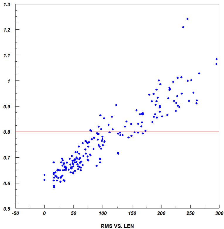
Figure 48: Electronic noise as function of trace length. The noise is measured in ADC counts and trace length length is in mm. The red line represents the maximum allowable noise based on the current TPC’s electronics.
