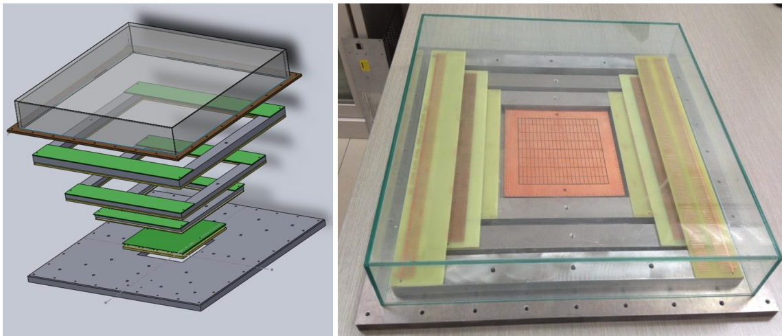
Figure 60: Exploded view and setup for the small scale MWPC prototype.
