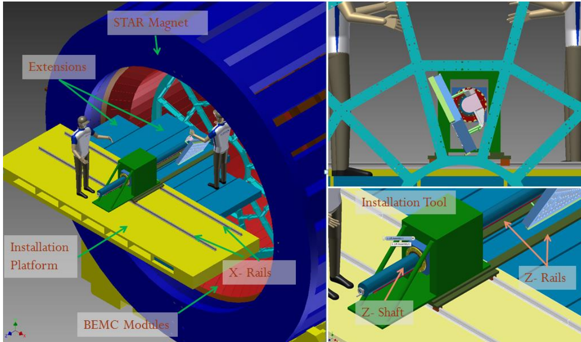
Figure 80: A conceptual design for a new sector insertion tool.
