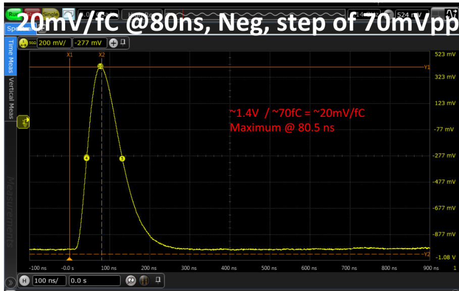
Figure 76: Output signal of the SAMPA preamplifier/shaper. Preliminary result of MWP1 "chip 1" evaluation
