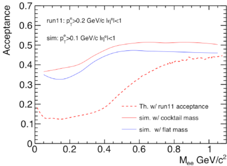
Figure 13: The electron acceptance using the current TPC (dashed red line) and the expected improvement using the iTPC under two different assumptions (red and blue lines).
