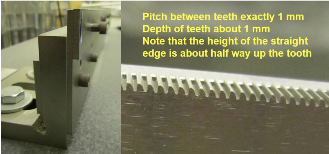
Figure 57: A wire comb mounted on the granite table in shown in the left hand figure. The “comb” is actually composed of two pieces; the comb and a straight edge. The figure on the right shows a close-up photo of the comb. The straight edge lies behind the comb and is located about half way up the teeth. The wires are aligned by being pushed into the corner defined by the intersection of the straightedge with the vertical sides of the comb.
