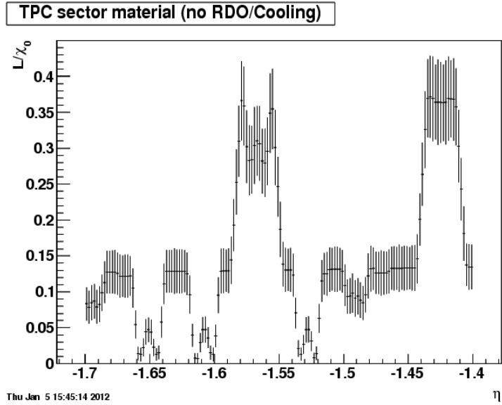
Figure 52: Radiation length vs. pseudorapidity for the original strongback. Electronics, cables and cooling manifolds are not included in these calculations. The lowest points are the cutouts for the electronics and so these numbers are not representative of the final assembly because this is where the FEE cards will sit and their average thickness is greater than 7%.
