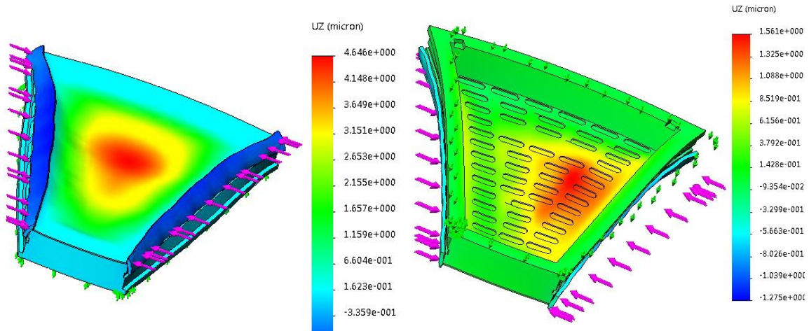
Figure 53: Simulated distortions in a proposed iTPC strongback due to the tension on the wire grids. The figure shows the result with the original rib design on the left, and without ribs on right. The maximum displacement of the padplane, with ribs, is 4.6 microns. The deformation of the padplane without ribs is less, only 1.6 microns. Summary: ribs are not needed to support the tension on the wires. Simulations courtesy of Howard Wieman.
