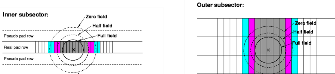
Figure 39: Simulations of the effective pad response function for pads on the inner and outer TPC padplanes. The inner pads were assumed to be 3.35 mm wide and the outer pads 6.7 mm wide. The circles show the 3-sigma limit for the pad response function convoluted with the diffusion limit for particles that drift the full distance from the CM to the padplane. P10 gas is assumed. The different circles show the different response that is recorded when the B field is set to 0.0, 0.25 T, or 0.5 T. [4]
