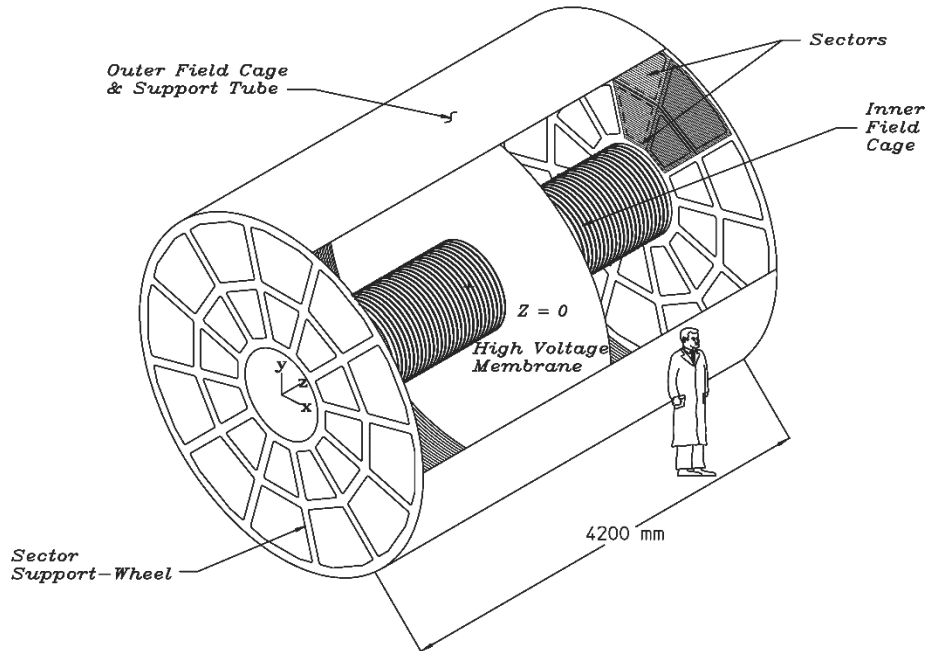
Figure 26: A schematic view of the STAR TPC. Secondary electrons drift away from the high voltage membrane, at the center, towards readout planes at either end of the TPC.
