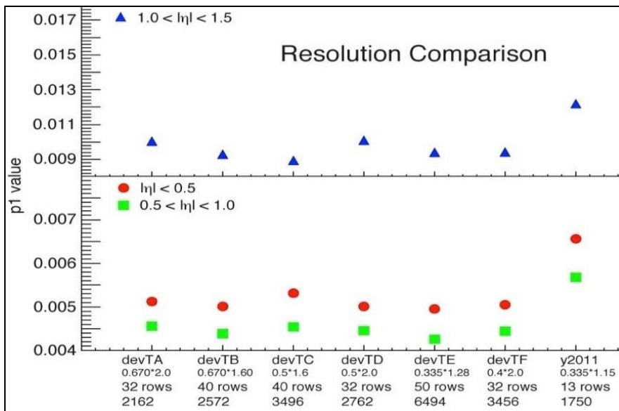
Figure 32: Track resolution (linear component) for different geometries of the inner part of the time projection chamber.
