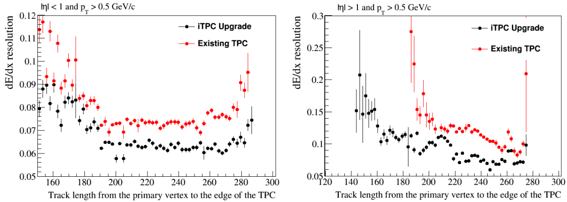
Figure 34: \frac{dE}{dx} resolution comparison for the existing and upgraded iTPC for two pseudorapidity regions.
