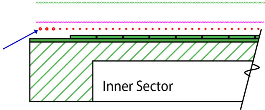
Figure 43: Three low gain wires (125 \mu\text{m} diameter) will be placed on both ends of the anode wire grid. The low gain wires will reduce the production of ions in the region where they can leak into the drift-volume of the TPC. Another option is to ground the last wire so that the gain is zero on that wire.
