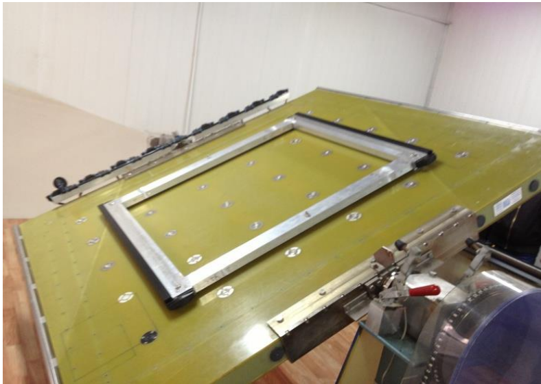
Figure 65: Wire winding on the first two wire planes with 20um W-wire.
