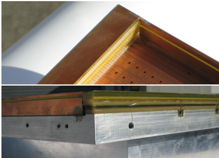
Figure 44: A top view and a side view of an ALICE inner readout chamber (iROC). The figures show one solution to the “grid leak” problem which is to terminate the plane of wires with a wall of G10 which has Cu traces that are biased appropriately to terminate the field lines coming from the anode wires and gated grid.
