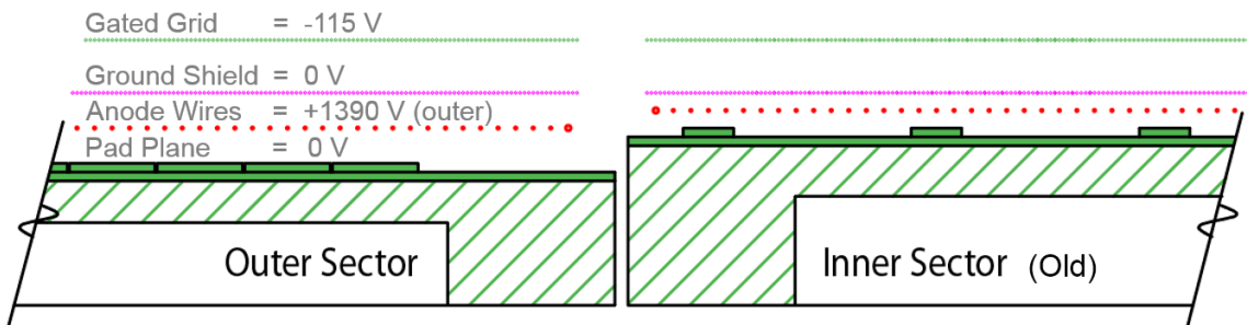
Figure 40: The original STAR pad plane geometry (side view). The outer sector pad rows covered the entire pad plane but the inner sector pad rows were widely spaced (> 5 cm).
