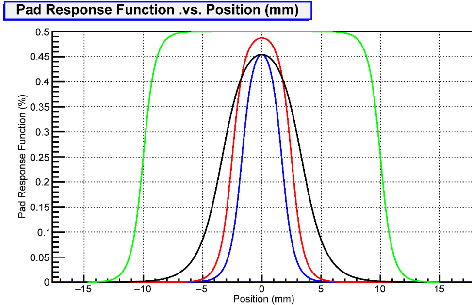
Figure 38: The pad response function for the outer sector is shown by the black line, the existing inner sector by the blue line, and the proposed inner sector by the red line. The pad spacing is 6.7 mm, 3.35 mm, and 5 mm respectively. The padplane to anode wire plane distance is 4 mm in the outer sector and 2 mm in the inner sector. The green line shows the PRF for a very wide pad, 20 mm, and it suggests that 50% of the signal goes to the padplane in the asymptotic limit. The diffusion width for an electron that drifts the full length of the TPC would be a curve that lies very close to the black line.
