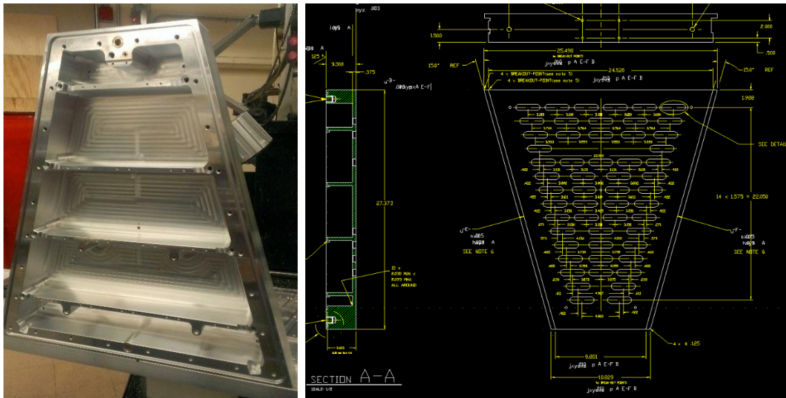
Figure 50: A prototype inner sector strongback is shown during fabrication at the University of Texas (circa 2013). The sector was machined out of a single piece of aluminum. Dimensions are: ~27 inches tall, ~25 inches wide and weight ~70 lbs. The sector is viewed from the backside.
