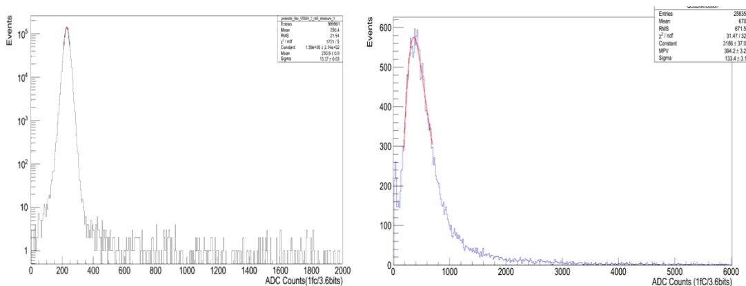
Figure 63: The pedestal measured on one pad at 1350 V (left) and the summed signal from all pads after pedestal subtraction (right).
