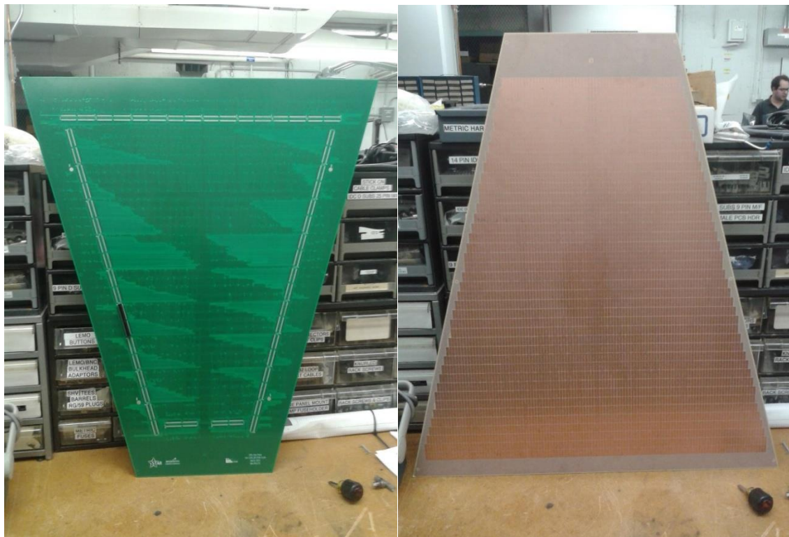
Figure 46: First padplane prototype. Left connector side. Right pad side.
