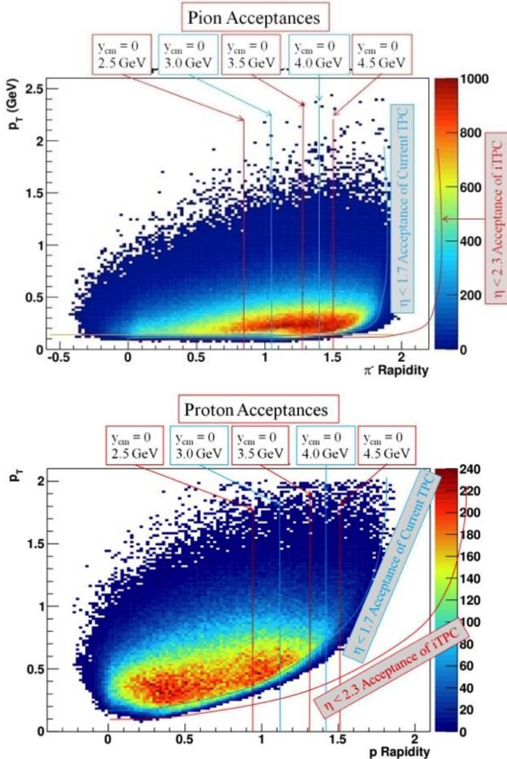
Figure 25: The acceptance for pions (top) and protons (bottom) in fixed-target mode. The histogram is filled with data from Au+Al background events taken during BES-I. The alternating red and cyan vertical bars indicate the center-of-mass rapidity for various energies to be studied. The cyan and red curves indicate the lower acceptance cut-ins for the current TPC and iTPC configurations, respectively.
