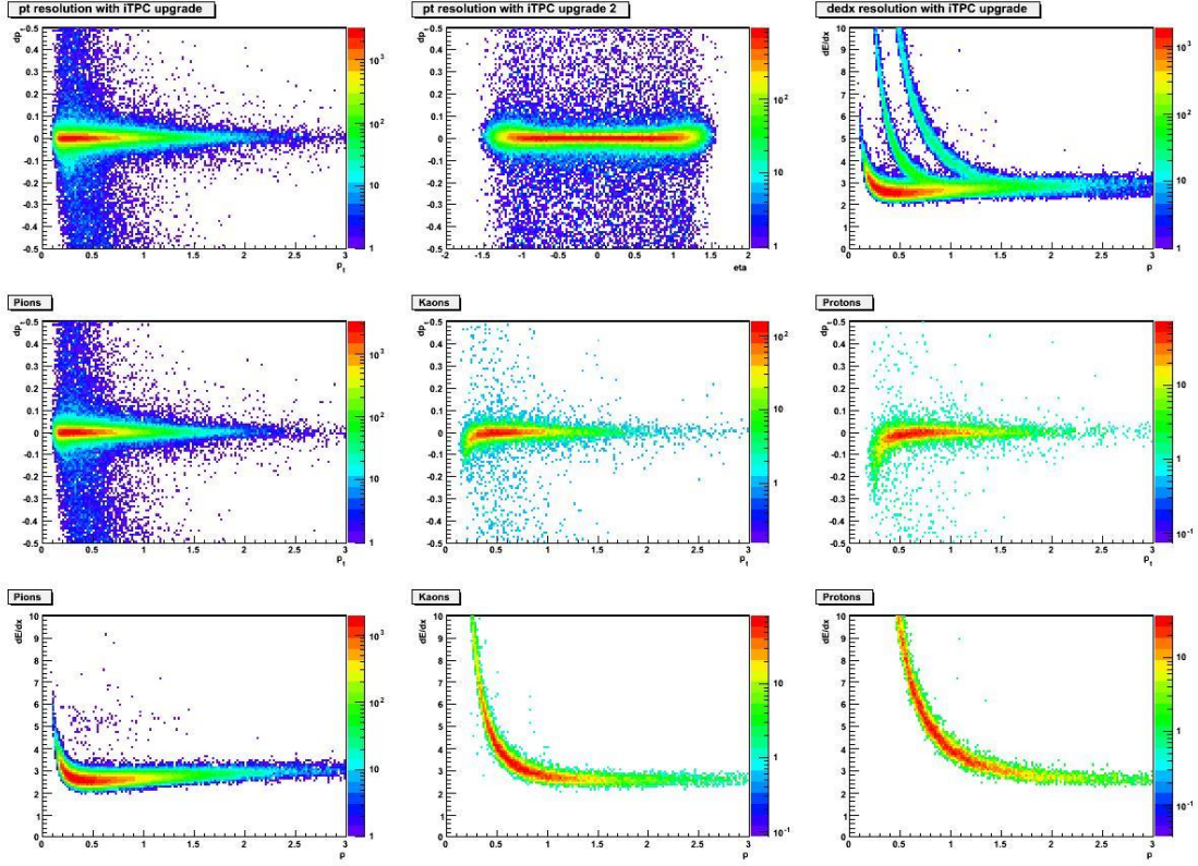
Figure 30: Characteristics of the reconstructed events simulated with the new iTPC geometry.
