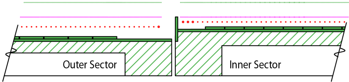
Figure 45: Two solutions to the Grid-Leak problem. Three low gain (or zero gain) wires on the end of the anode grid help to reduce production of ions in this region, and the vertical wall terminates the field lines so that positive ions produced in this region cannot leak out into the gap between the inner and outer sectors.
