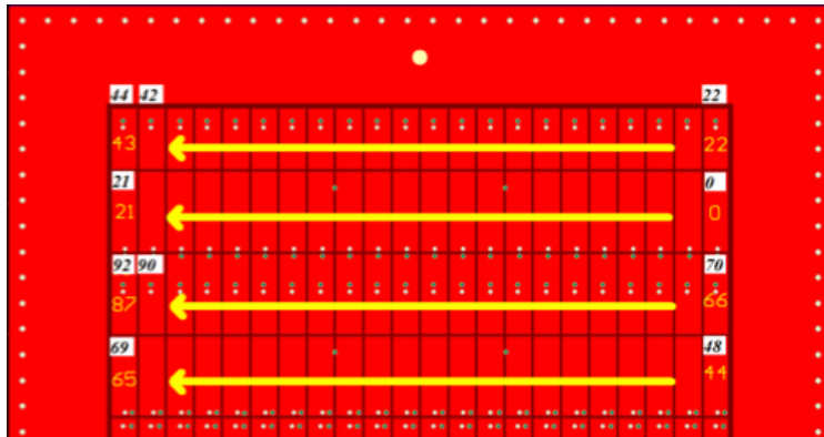
Figure 62: Pad numbering scheme for the small MWPC prototype.
