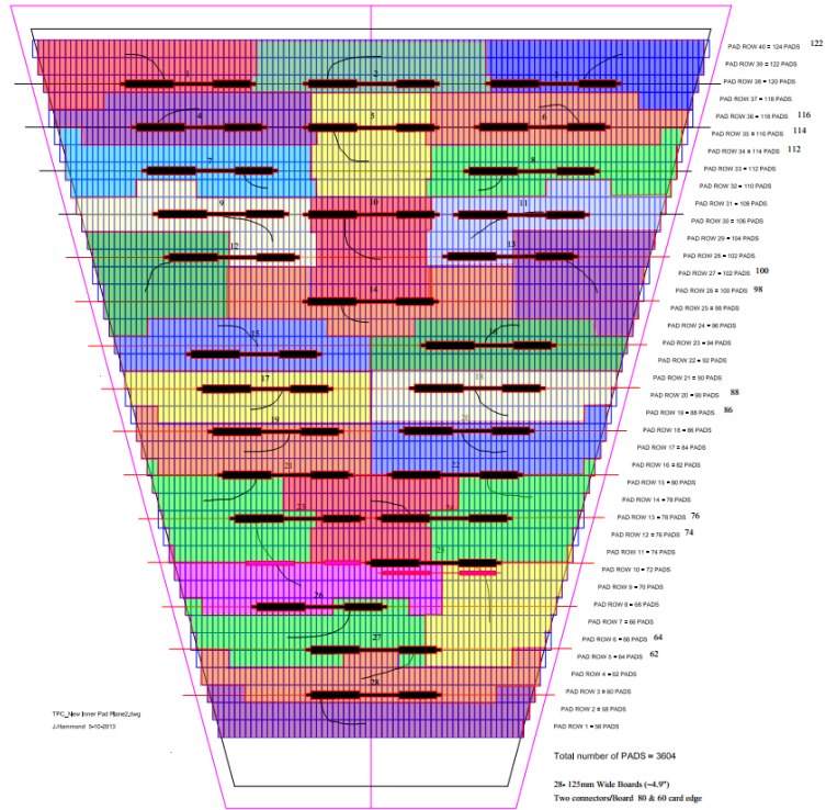
Figure 49: The new padplane design
