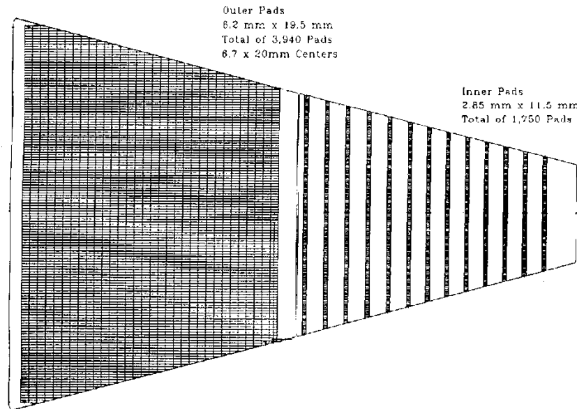
Figure 27: Configuration of the existing pad rows in a STAR TPC padplane super-sector (one inner sector and one outer sector). Note that the outer sector padplane coverage is complete but the inner sector pad rows do not cover the full area of the inner sector.
