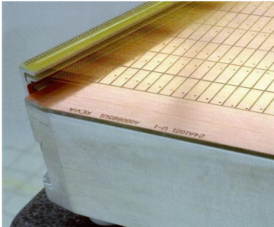
Figure 36: A photo of an outer sector padplane showing the MWPC, the padplane, and the Aluminum strongback that supports the padplane and wire grids. The MWPCs are really three grids of wires; the gated grid (top), the ground grid (middle, also known as the cathode grid), and the anode wires (bottom).
