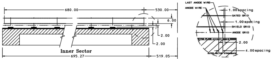
Figure 37: Side view of an inner sector adplane, strongback and wire grids. Dimensions are in mm.
