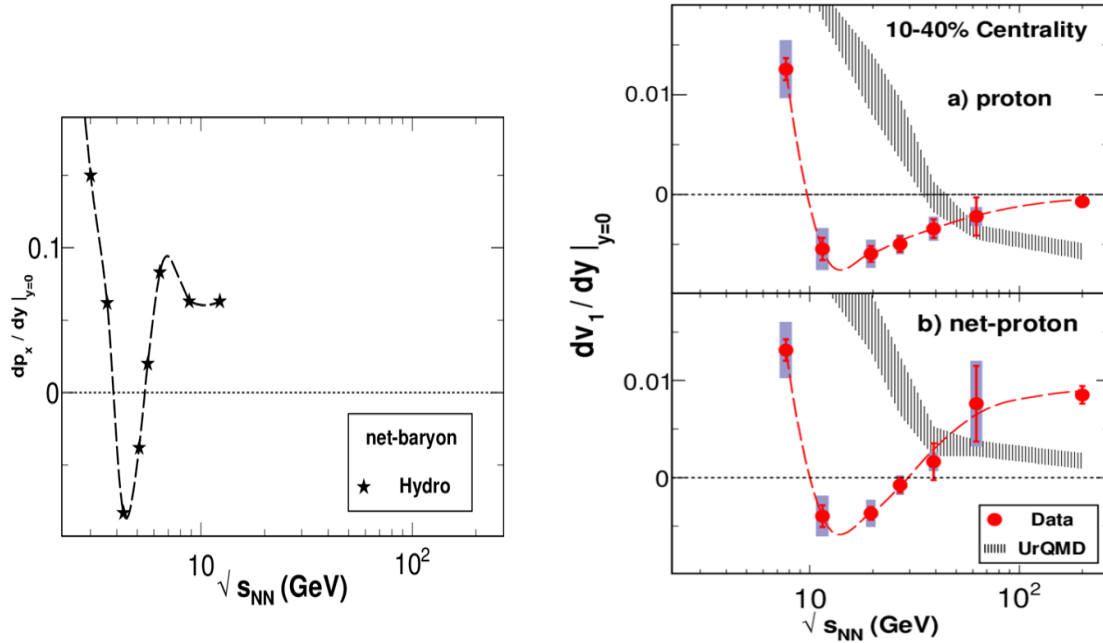
Figure 16: Left: Directed flow prediction in units of GeV/c as a function of beam energy, based on a three-fluid hydrodynamic model [3] whose EOS incorporates a first-order phase transition. Right: panel a) shows the slope of directed flow vs. beam energy for protons from Au+Au collisions at intermediate centrality. Panel b) presents the same for net protons. The prediction of the UrQMD transport model [6] is also plotted in panels a) and b).
