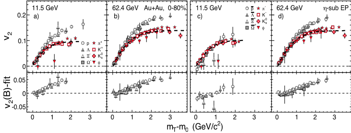
Figure 21: The upper panels depict the elliptic flow, v_2 , as a function of reduced transverse mass, m_T - m_0 , for particles (panels a and b), and for antiparticles (panels c and d), in 0-80% central Au+Au collisions at \sqrt{s_{NN}} = 11.5 and 62.4 GeV. Simultaneous fits to mesons other than pions are shown as dashed lines. The difference between the baryon v_2 and the meson fits are shown in the lower panels.
