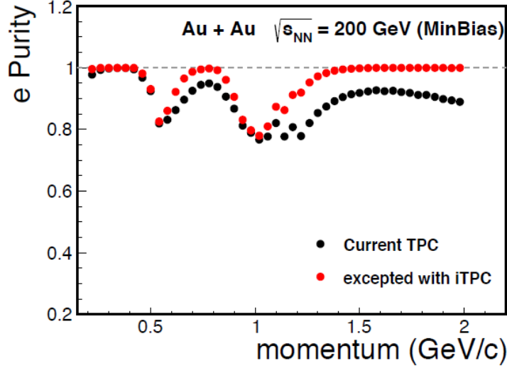
Figure 12: The expected purity for electrons as a function of transverse momentum. The black symbols show the purity using the current TPC. The improved purity with the iTPC is shown in red symbols.
