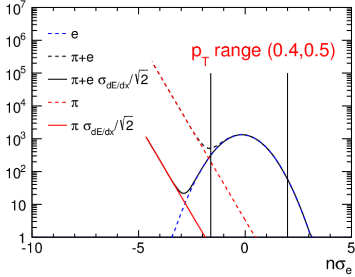
Figure 10: dE/dx of electrons and hadron background, as a function of n\sigma_e , for 0.4 < p_T < 0.5 GeV/c. The blue Gaussian curve is the electron dE/dx while the red dashed line is a fit to the measured hadron dE/dx tail. The solid red line is the expected hadron contamination with the improved tracking of the iTPC.
