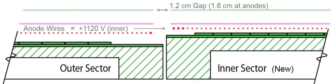
Figure 41: The new STAR pad plane geometry. The outer sector configuration remains the same, but the inner sector has more pad rows and there aren't any gaps between the pad rows.
