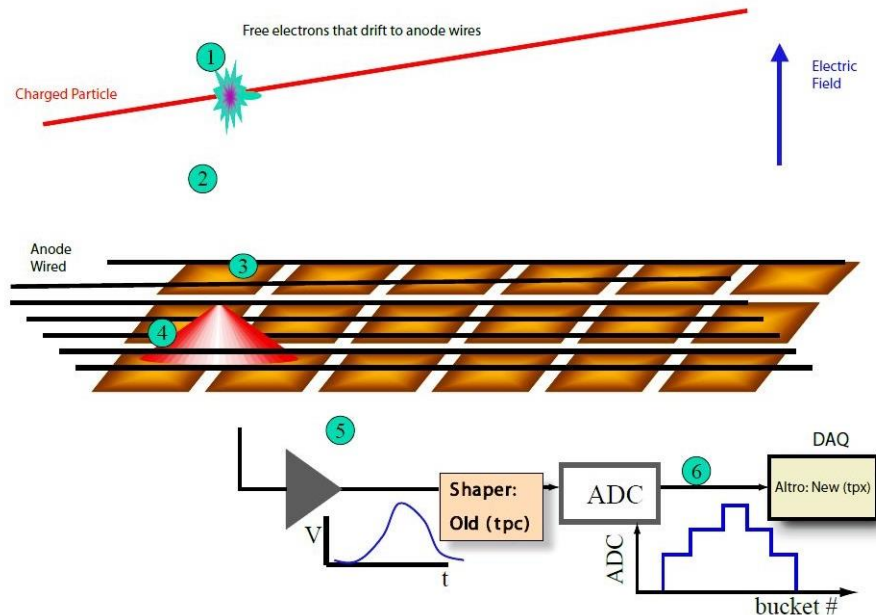
Figure 29: Schematic view of the TPC response simulator flow chart.
