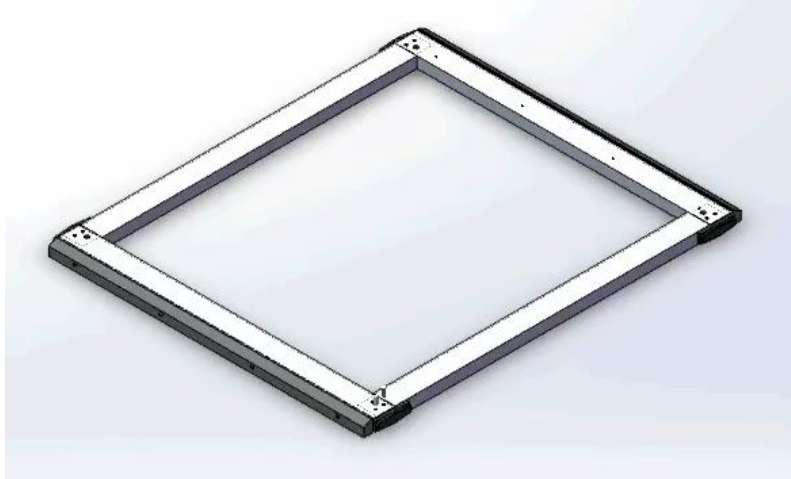
Figure 64: A sketch of the temporary wire transfer frame. The inner size for the box is 76.2 x 90.0 cm and the size of the material is 3.0 x 6.0 x 0.3 cm.
