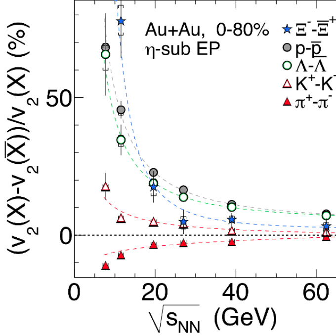
Figure 20: The difference in v_2 between particles and their antiparticles (see legend) as a function of \sqrt{s_{NN}} for 0-80% central Au+Au collisions. The dashed lines are fits with a power-law function. The error bars depict the combined statistical and systematic errors.
