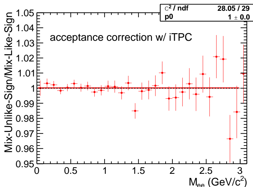
Figure 14: The acceptance difference factor, the ratio of the mixed-event unlike-sign to the mixed-event like-sign electron pair invariant mass distributions with the iTPC upgrade.
