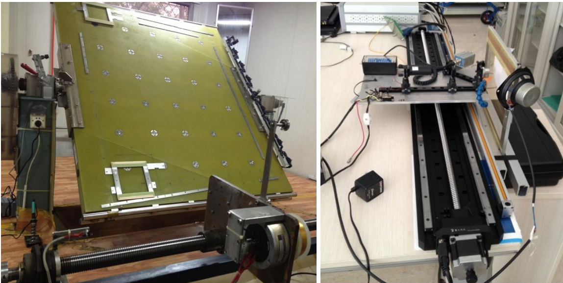
Figure 59: The wire winding machine at SDU (left) and the optical system for making wire tension measurements (right).
