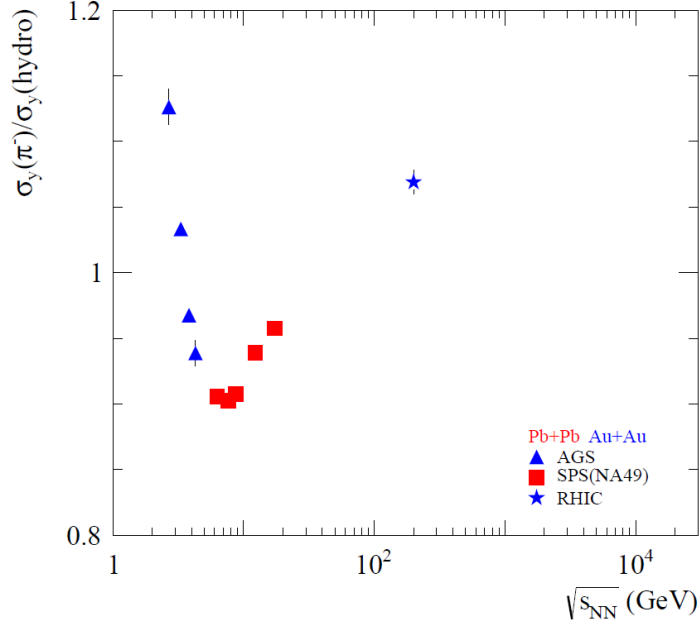
Figure 19: The width of pion rapidity distributions [11], normalized to calculations based on Landau’s hydrodynamic model [9] as a function of beam energy. The minimum may be an indication of the softening of the EoS [10,11]. The only available RHIC measurement to date is at \sqrt{s_{NN}} = 200 GeV, from BRAHMS [12].
