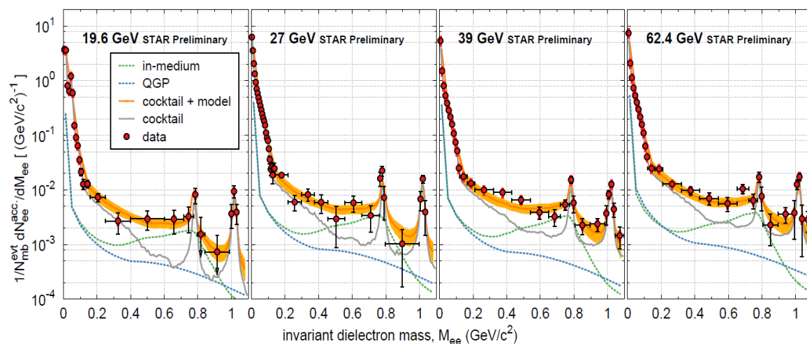
Figure 7: Preliminary STAR measurements of dielectron invariant mass distributions below 1.1 \text{ GeV}/c^2 for \sqrt{s_{NN}} = 19.6, 27, 39 and 62.4 GeV. The grey cocktail curve includes all known hadronic sources apart from the \rho (which is included in the model). The orange band includes a model calculation [29] with contributions from both hadron gas and QGP phases.
