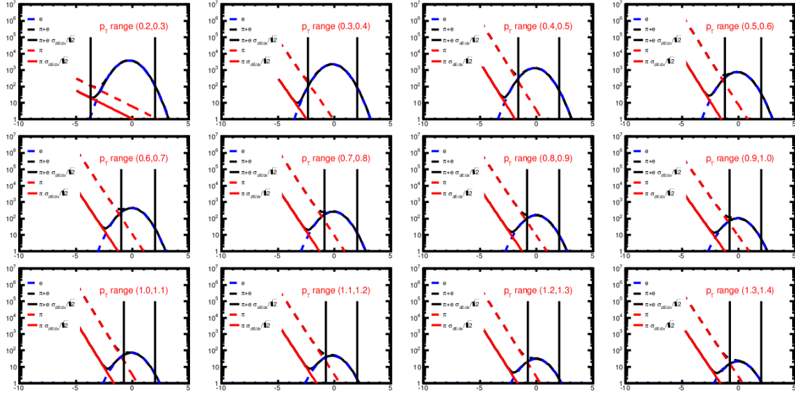
Figure 11: These panels demonstrate the iTPC improvement for 12 different p_T intervals, following the same scheme as plotted in the previous figure.
