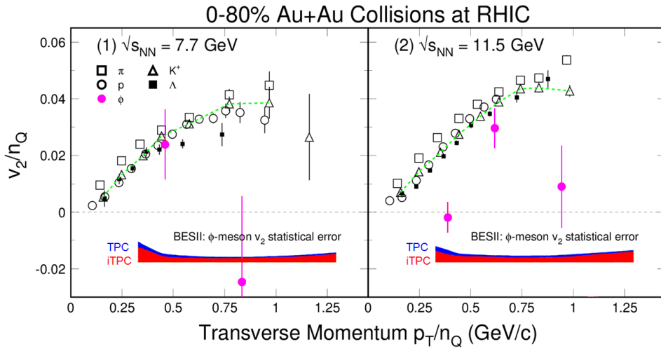
Figure 23: Scaled v_2 of the phi meson showing the projected error bars for BESII with the current TPC (blue band) and with the iTPC (red band).
