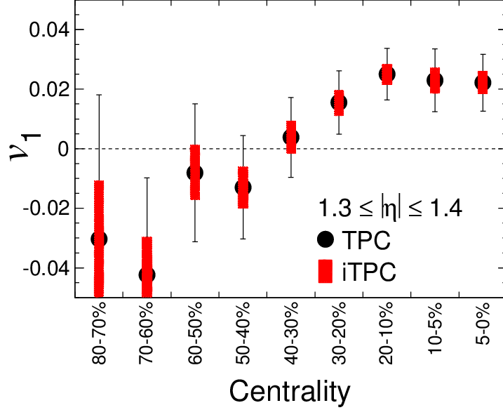
Figure 18: The Forward v_1 measurement as a function of centrality explicitly showing the improvements due to the coverage of the iTPC.
