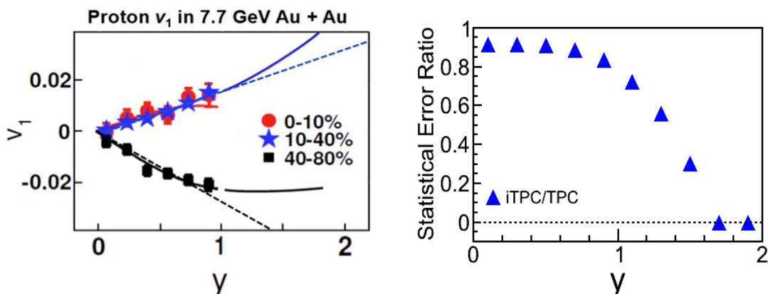
Figure 17: Left: Plotted points show measured directed flow v_1(y) for protons in three centrality bins for Au+Au collisions at \sqrt{s_{NN}} = 7.7 GeV. The solid curves are a cubic fit to the measured data points for intermediate and peripheral centralities while the dashed lines are linear fits. These fits are extrapolated into the rapidity region that will become accessible after the iTPC upgrade. For simplicity, only positive rapidities are plotted here. Right: The improvement in statistical errors that would be achieved with the iTPC upgrade, for directed flow measurements at low RHIC energies as a function of rapidity, for any fixed number of events, based on simulations using the UrQMD model. Positive and negative rapidities give the same result, and are averaged in this plot. The two high rapidity points where a zero ratio is plotted correspond to acceptance regions where the present TPC provides no data whatsoever.
