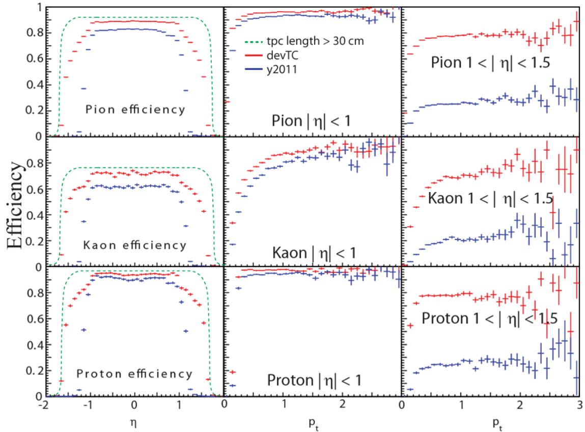
Figure 33: Efficiency of pion, kaon, and proton measurements as a function of pseudorapidity and transverse momentum (in GeV/c) for the current TPC design (blue) and for the devTC design (red). The theoretical curve for the efficiency for tracks longer than 30 cm is shown as a green dashed line.
