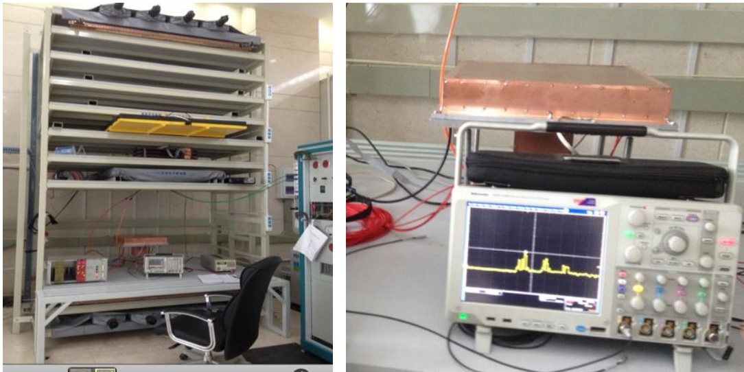
Figure 61: The cosmic ray test stand at SDU and associate test equipment.
