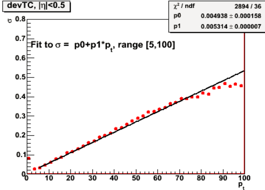
Figure 31: Momentum resolution as a function of the transverse momentum to extract the p1 value.
