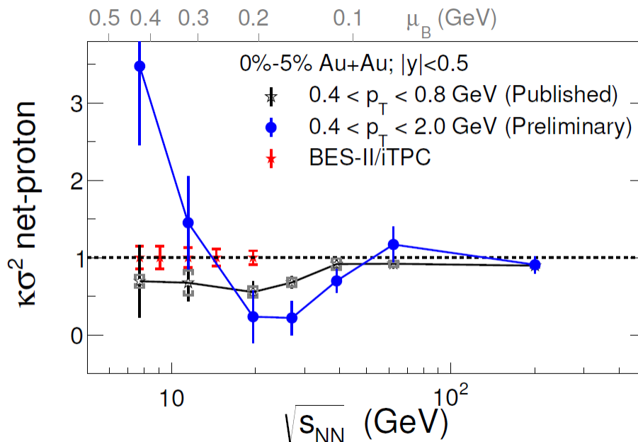
Figure 4: The left panel shows the effects of p_T selections on the \kappa\sigma^2 signal and the projected errors for BESII.
