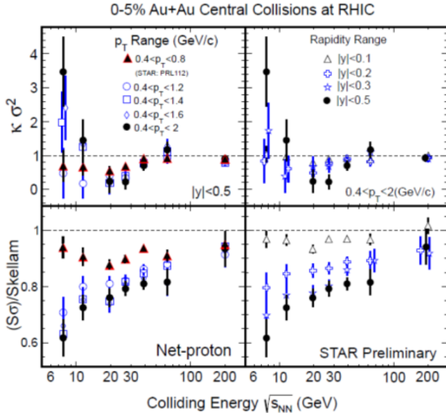
Figure 3: STAR results for beam energy dependence of \kappa\sigma^2 (top panels) and S\sigma/\text{Skellam} (lower panels) for net protons [18] in Au+Au collisions. The left panel illustrate the effect of p_T selections while the right panels indicate the effects of rapidity selections. Dotted horizontal lines are expectations from Poisson distributions.
