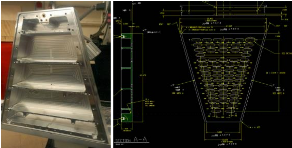
Figure 51: A prototype inner sector strongback is shown during fabrication at the University of Texas (circa 2013). The sector was machined out of a single piece of aluminum. Dimensions are: ~27 inches tall, ~25 inches wide and weight ~70 lbs. The sector is viewed from the backside.
