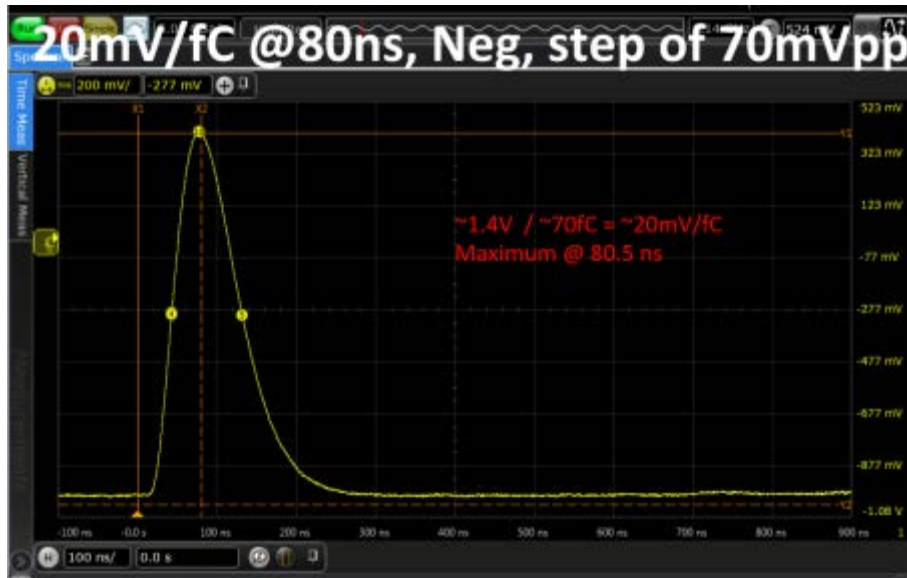
Figure 88: Output signal of the SAMPA preamplifier/shaper. Preliminary result of MWP1 "chip 1" evaluation
