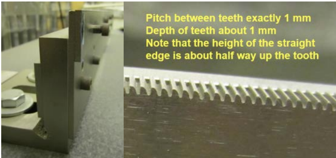
Figure 58: A wire comb mounted on the granite table in shown in the left hand figure. The “comb” is actually composed of two pieces; the comb and a straight edge. The figure on the right shows a close-up photo of the comb. The straight edge lies behind the comb and is located about half way up the teeth. The wires are aligned by being pushed into the corner defined by the intersection of the straightedge with the vertical sides of the comb.
