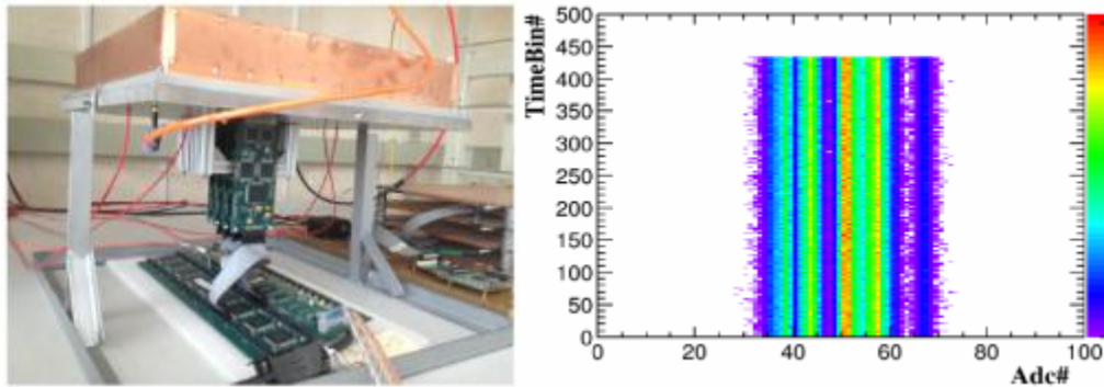
Figure 69: (Left): the connection between small prototype, FEEs and RDO board. (Right): the ADC value versus the time bin number
