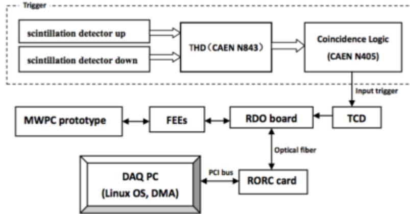
Figure 66: Layout of the MWPC prototype test system.
