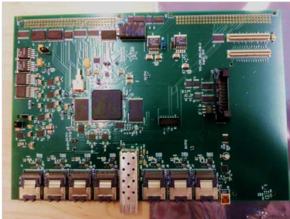
Figure 90: iRDO prototype.
