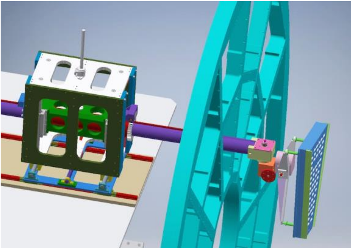
Figure 95: Schematic views of the sector manipulation tool placing an inner sector assembly through the opening at the 12 o'clock position of the TPC end-wheel.
