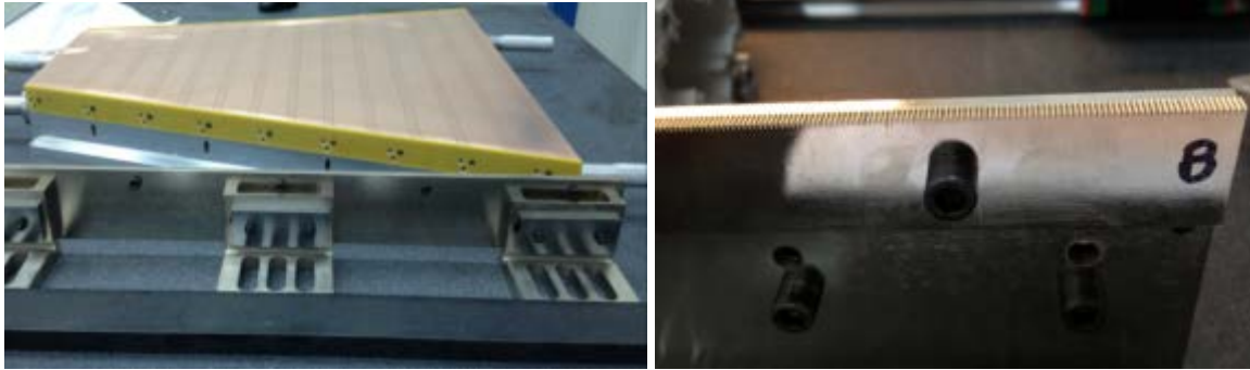
Figure 81: One side the wire combs installed including angle plates, straight edge and combs (left), and a zoomed view for the combs and straight edge..
