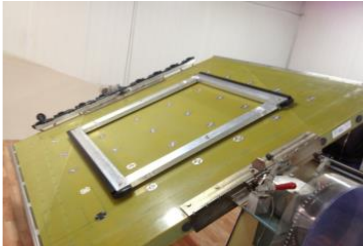
Figure 71: Wire winding on the first two wire planes with 20um W-wire.
