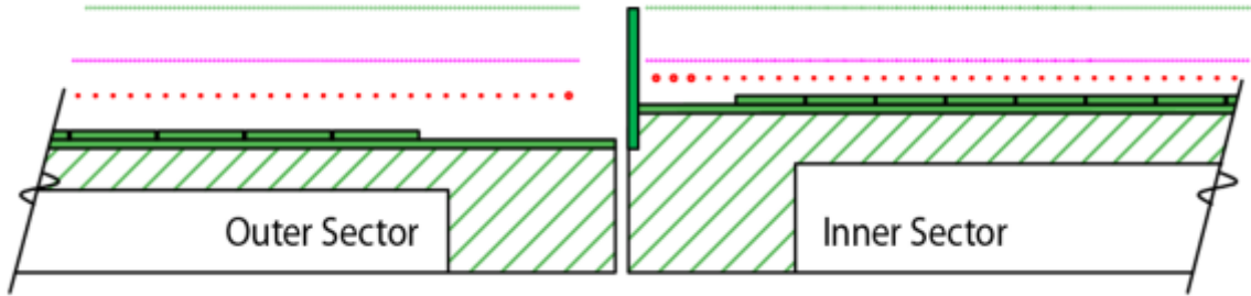
Figure 46: Two solutions to the Grid-Leak problem. Three low gain (or zero gain) wires on the end of the anode grid help to reduce production of ions in this region, and the vertical wall terminates the field lines so that positive ions produced in this region cannot leak out into the gap between the inner and outer sectors.
