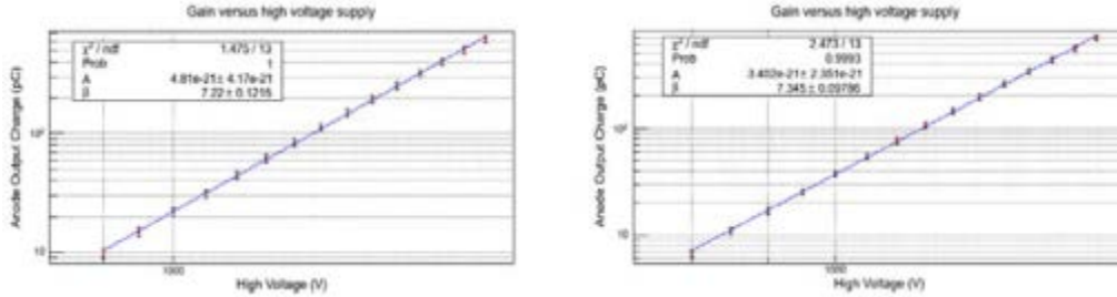
Figure 68: the anode output charge versus high voltage supply of Hamamatsu R11102-A52468 (left) and R11102-A52723 (right).
