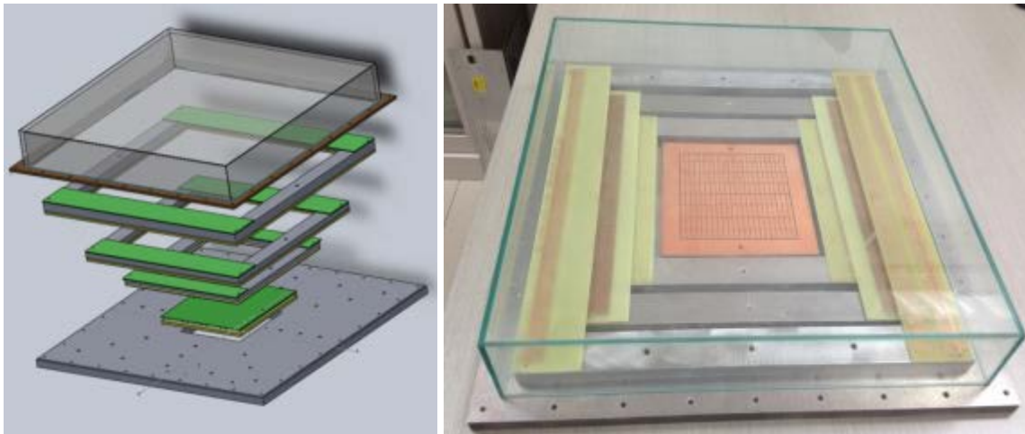
Figure 62: Exploded view and setup for the small scale MWPC prototype.
