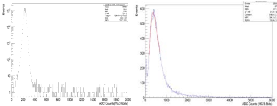
Figure 65: The pedestal measured on one pad at 1350 V (left) and the summed signal from all pads after pedestal subtraction (right).
