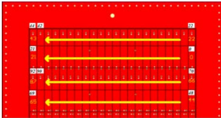
Figure 64: Pad numbering scheme for the small MWPC prototype.
