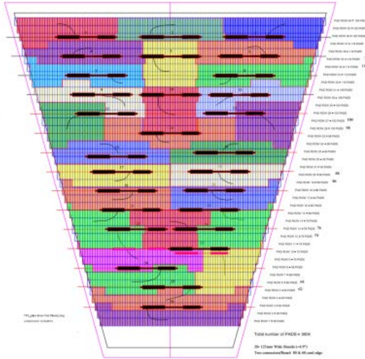
Figure 50: The new padplane design
