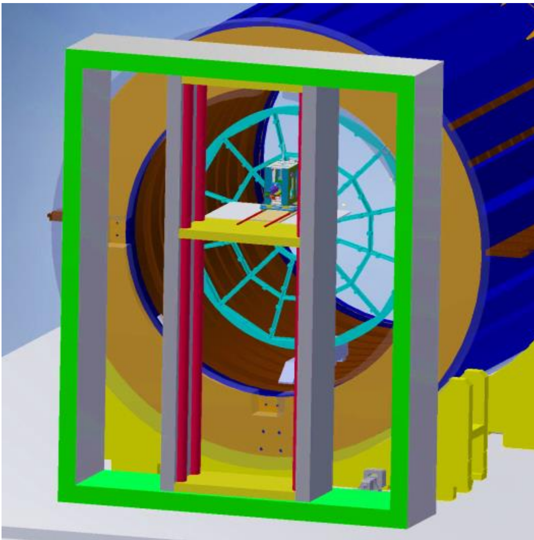
Figure 92: Schematic diagram of the proposed new sector-mounting tool. The green walls are fixed to the magnet face and define the limits of motion in the plane parallel to the TPC end-wheel. The red support columns move horizontally within the green walls and the lift that supports the sector manipulation tool moves vertically on red columns.
