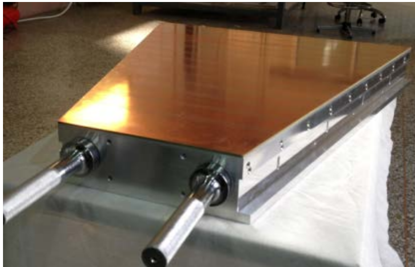
Figure 74: The strongback with the pad plane glued.
