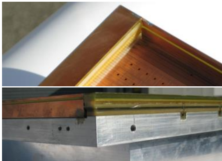
Figure 45: A top view and a side view of an ALICE inner readout chamber (iROC). The figures show one solution to the “grid leak” problem which is to terminate the plane of wires with a wall of G10 which has Cu traces that are biased appropriately to terminate the field lines coming from the anode wires and gated grid.
