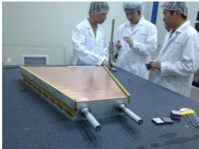
Figure 78: Strongback with all three side wire mounts attached before drilling/pinning.
