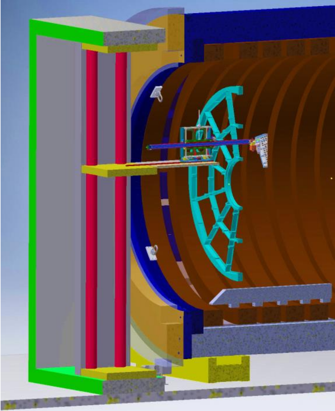
Figure 94: Cross sectional schematic view of the platform to show how the sector manipulation tool sits on the lift.
