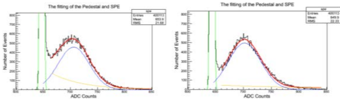
Figure 67: the SPE spectrum of Hamamatsu R11102-A52468(left) and R11102-A52723(right)
