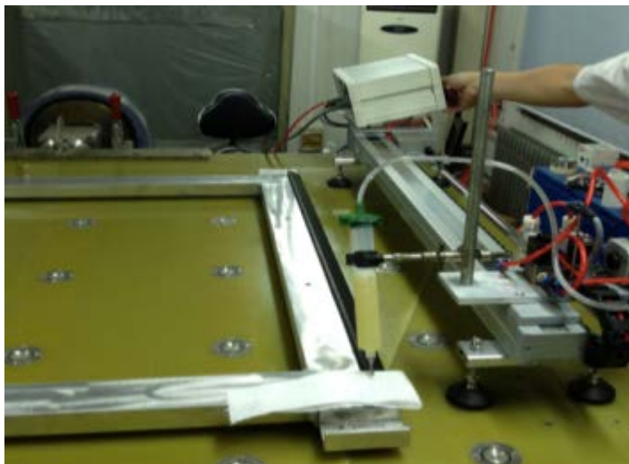
Figure 72: Gluing robot for dispensing epoxy on thin edges
