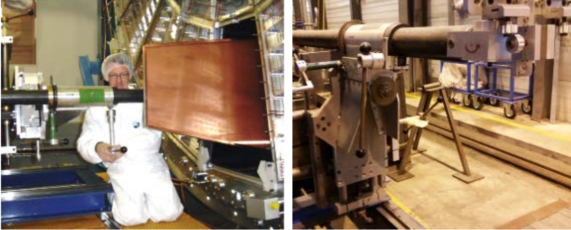
Figure 96: Photographs of the TPC sector manipulation tool used in assembly of the ALICE TPC at LHC.
