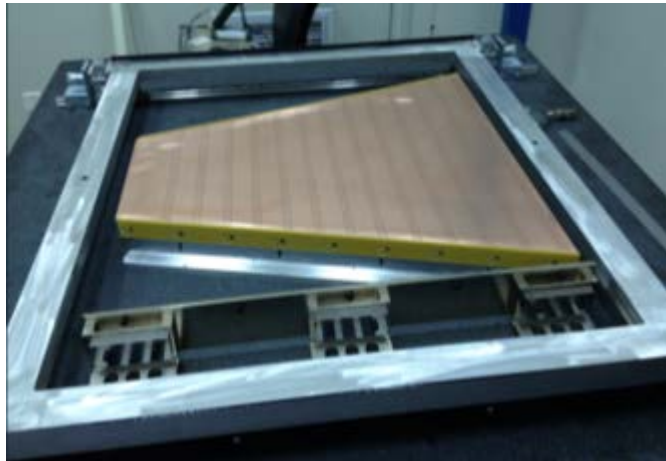
Figure 82: Putting the wire frame on the wire combs
