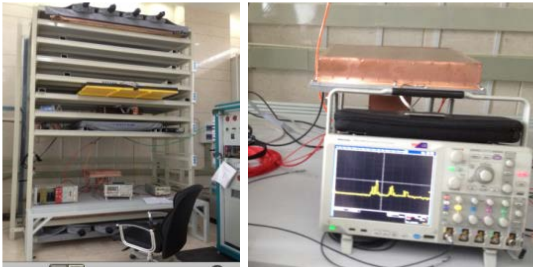
Figure 63: The cosmic ray test stand at SDU and associated test equipment.
