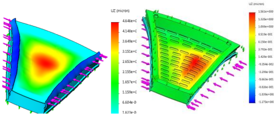
Figure 54: Simulated distortions in a proposed iTPC strongback due to the tension on the wire grids. The figure shows the result with the original rib design on the left, and without ribs on right. The maximum displacement of the padplane, with ribs, is 4.6 microns. The deformation of the padplane without ribs is less, only 1.6 microns. Summary: ribs are not needed to support the tension on the wires. Simulations courtesy of Howard Wieman.
