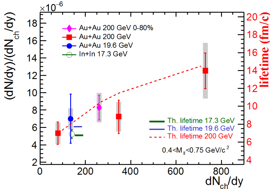
Figure 10: Integrated yields of the normalized dilepton excesses for 0.4 < M_{||} < 0.75 \text{ GeV}/c^2 as a function of dN_{ch}/dy . The solid circle and diamond represent the results in 0-80% Au+Au collisions at \sqrt{s_{NN}} = 19.6 and 200 GeV, respectively. The squares are the results for 40-80%, 10-40%, and 0-10% Au+Au at \sqrt{s_{NN}} = 200 GeV. The open circle represents the dimuon result from the NA60 measurement with dN_{ch}/dy > 30 . Bars are statistical uncertainties, and systematic uncertainties are shown as grey boxes. The theoretical lifetimes for \sqrt{s_{NN}} = 200 GeV Au+Au as a function of dN_{ch}/dy in the model calculations [37] are shown as a dashed curve. The lifetimes for \sqrt{s_{NN}} = 17.3 GeV In+In and \sqrt{s_{NN}} = 19.6 GeV Au+Au in the same model calculations [37] are shown as the two horizontal bars. The dN_{ch}/dy values for the horizontal bars are shifted for clarity.
