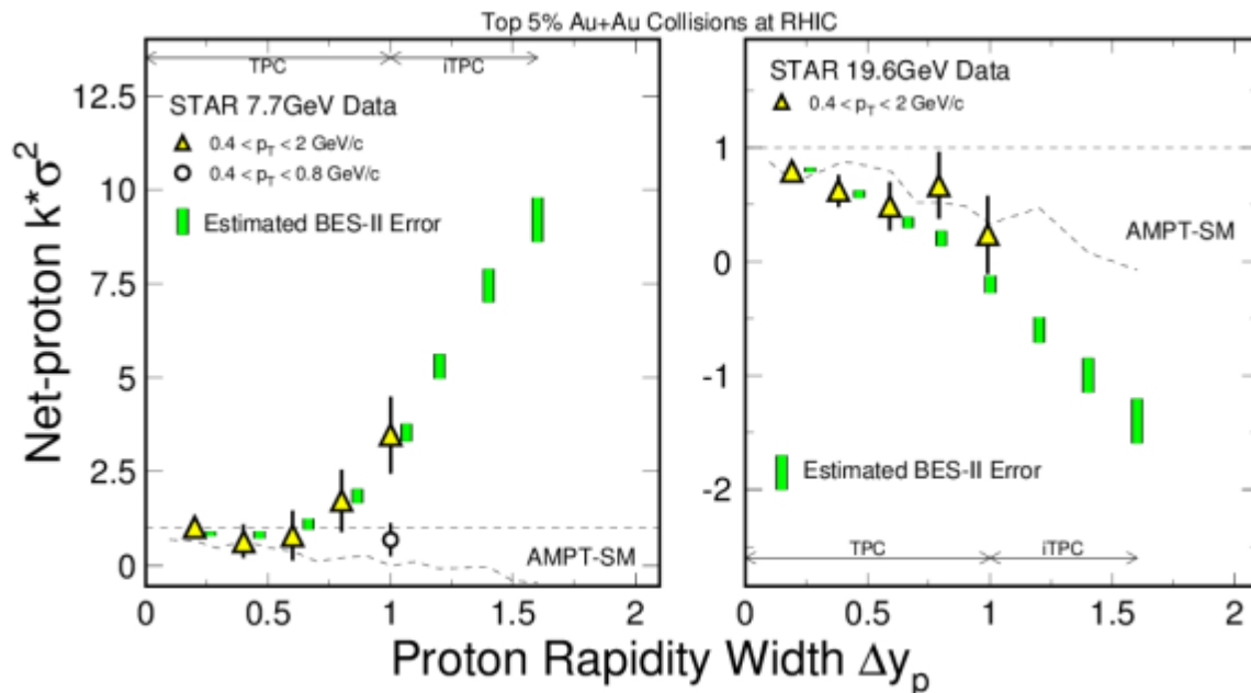
Figure 2: The observed net-proton kurtosis ( \kappa \cdot \sigma^2 ) as a function of rapidity window from BES I (yellow triangles). These preliminary data are for central (5%) Au+Au collisions at 7.7 GeV (left panel) and 19.6 GeV (right panel). The green bars are the estimated statistical uncertainties with the iTPC for BES-II, for 7.7 GeV and 19.6 GeV. In the extended region covered by the iTPC upgrade ( 1.0 < |\Delta y| < 1.6 ), the error bars were estimated assuming that the variances increase linearly with rapidity width. The locations of the projected error bars illustrate one possible rapidity-window dependence of the net-proton Kurtosis signal. Also shown are AMPT simulations with string melting and without a critical point (dashed lines).
