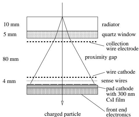
Fig. 1. Cutaway view of the detector[2].
