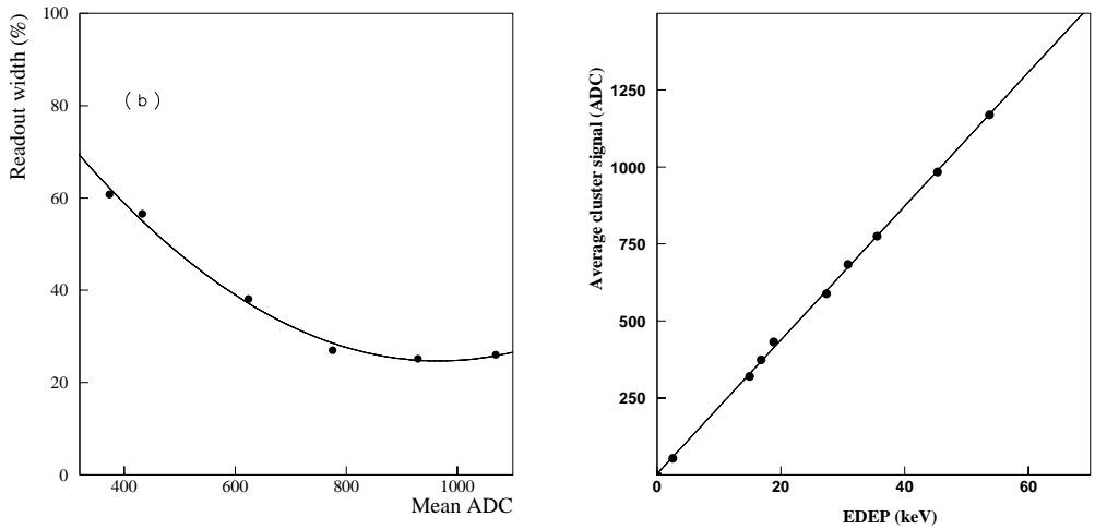
Fig. 11. (left) Readout width (%) shown for various energy deposition expressed in terms of cluster ADC, (right) Calibration plot, showing the relation between the energy deposition obtained from simulation and the cluster ADC obtained from test data.
