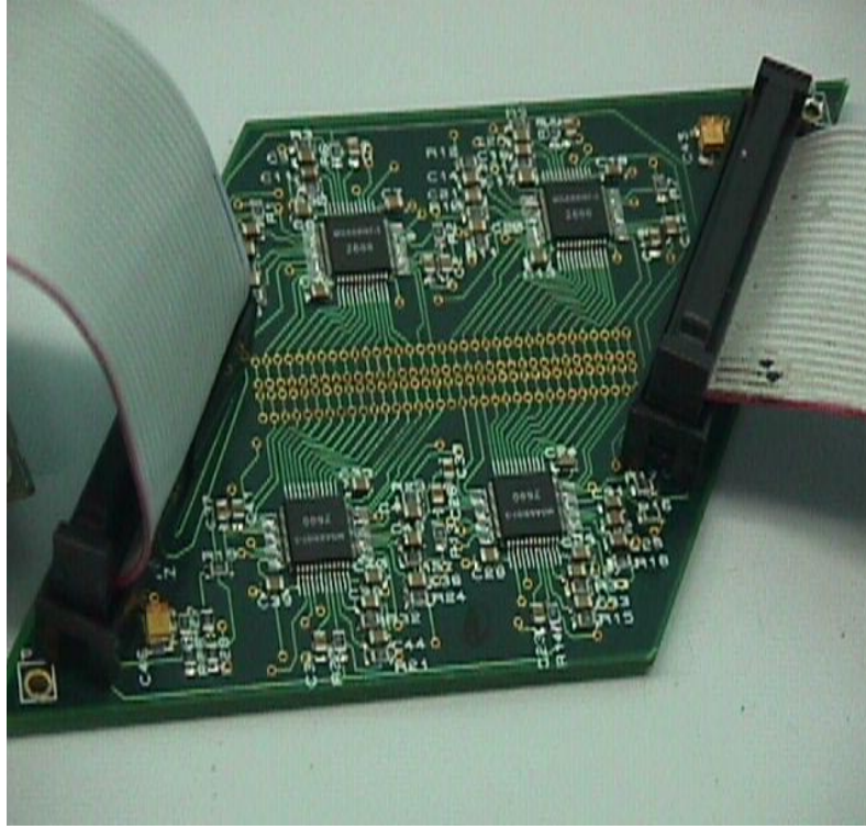
Fig. 6. Photograph of a FEE board with four GASSIPLEX chips.
