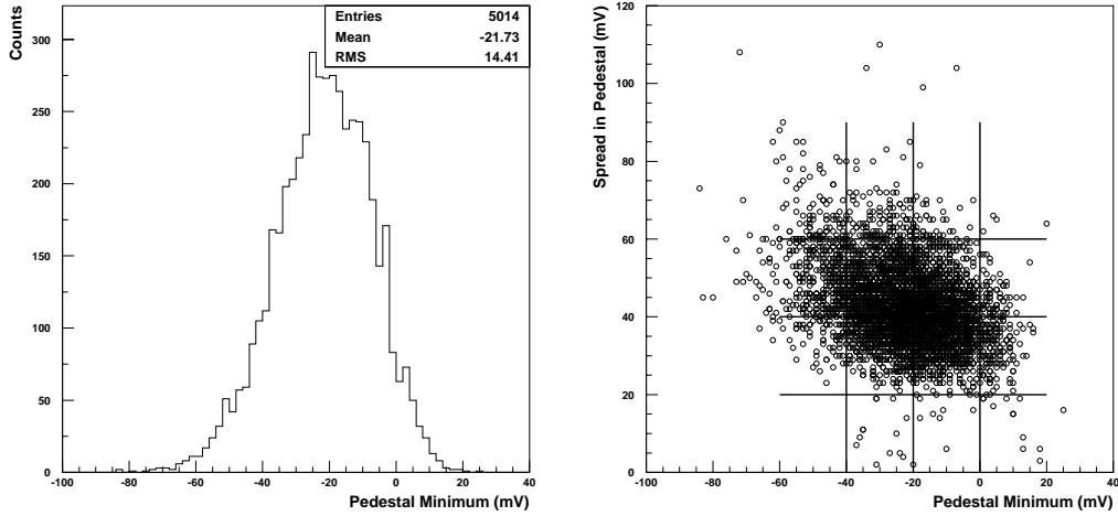
Fig. 7. (a) Pedestal minimum values ( in mV) for 5000 chips, (b) pedestal minimum vs. pedestal spread for these chips. Lines are drawn to suggest the grouping of chips for a uniform chain.
