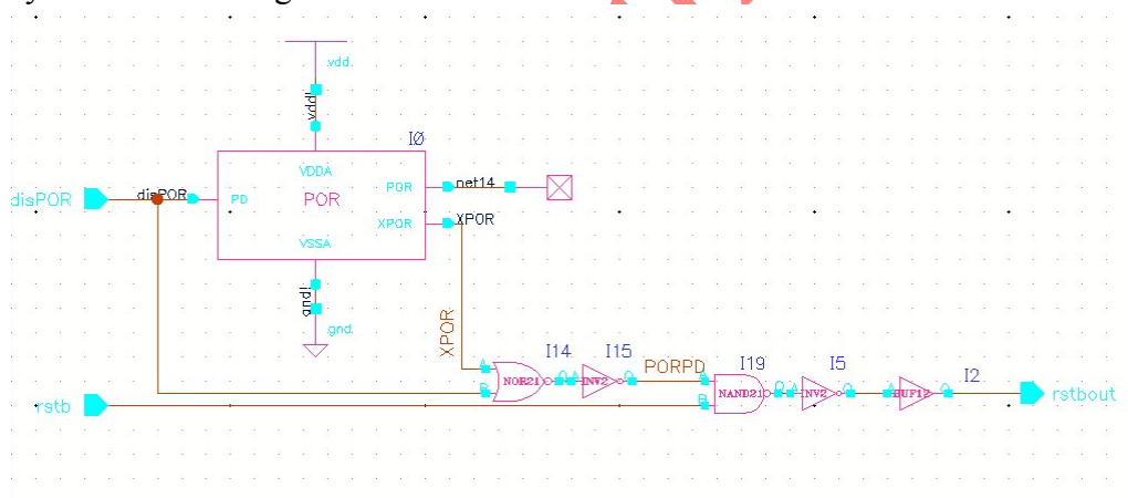
a) Schematic of Power On Reset
